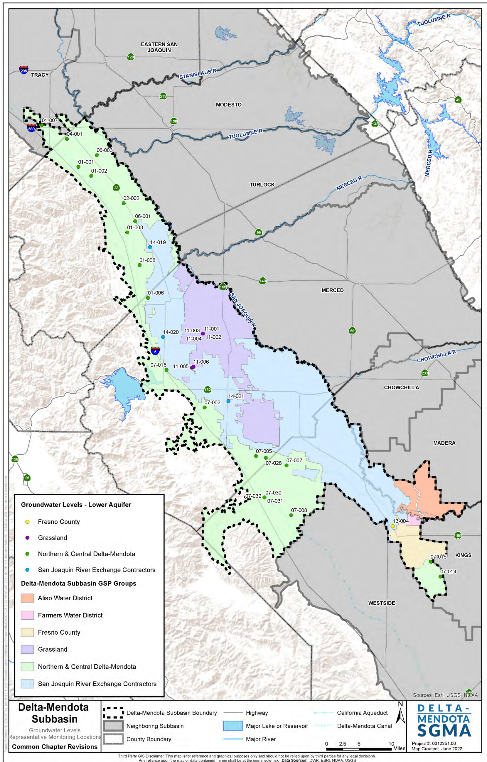
Figure 7-3. Groundwater Level Monitoring Network, Lower Aquifer
