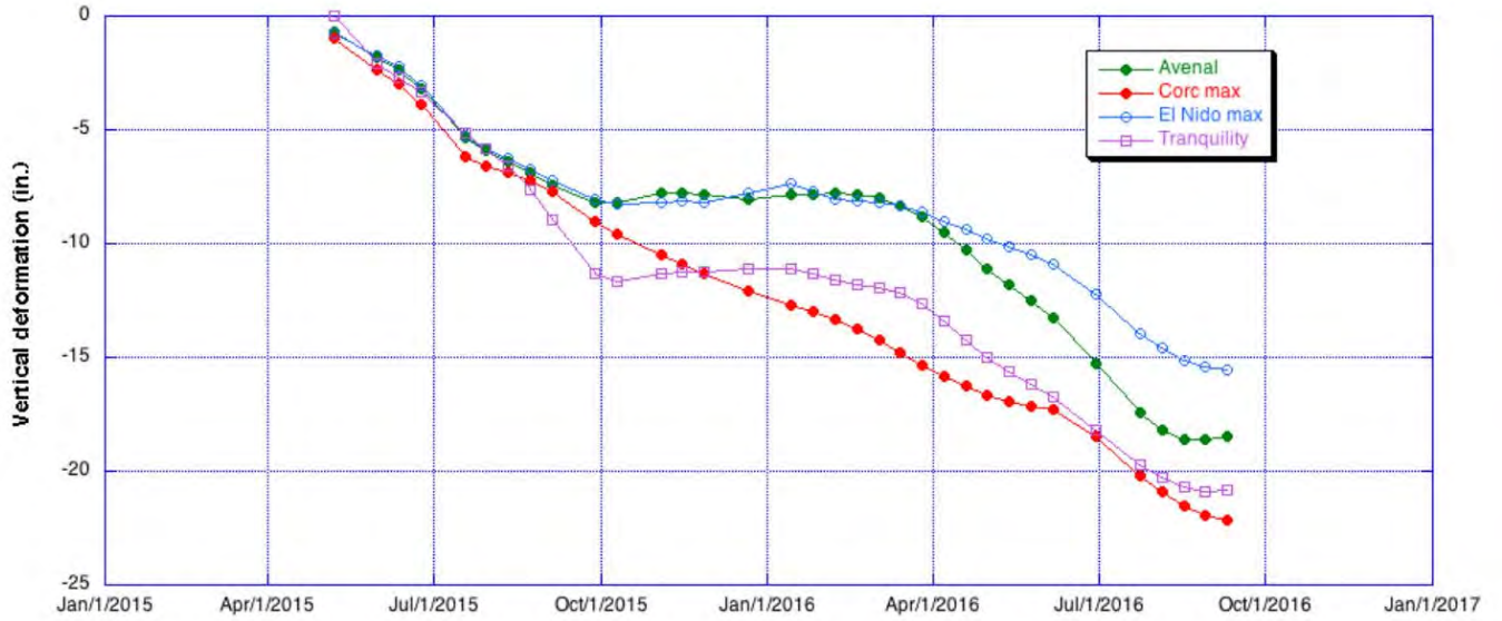
Figure 5-115. Recent Land Subsidence at Key San Joaquin Valley Locations (Source: Progress Report: Subsidence in California, March 2015 – September 2016 , Farr et. al. JPL, 2017)
